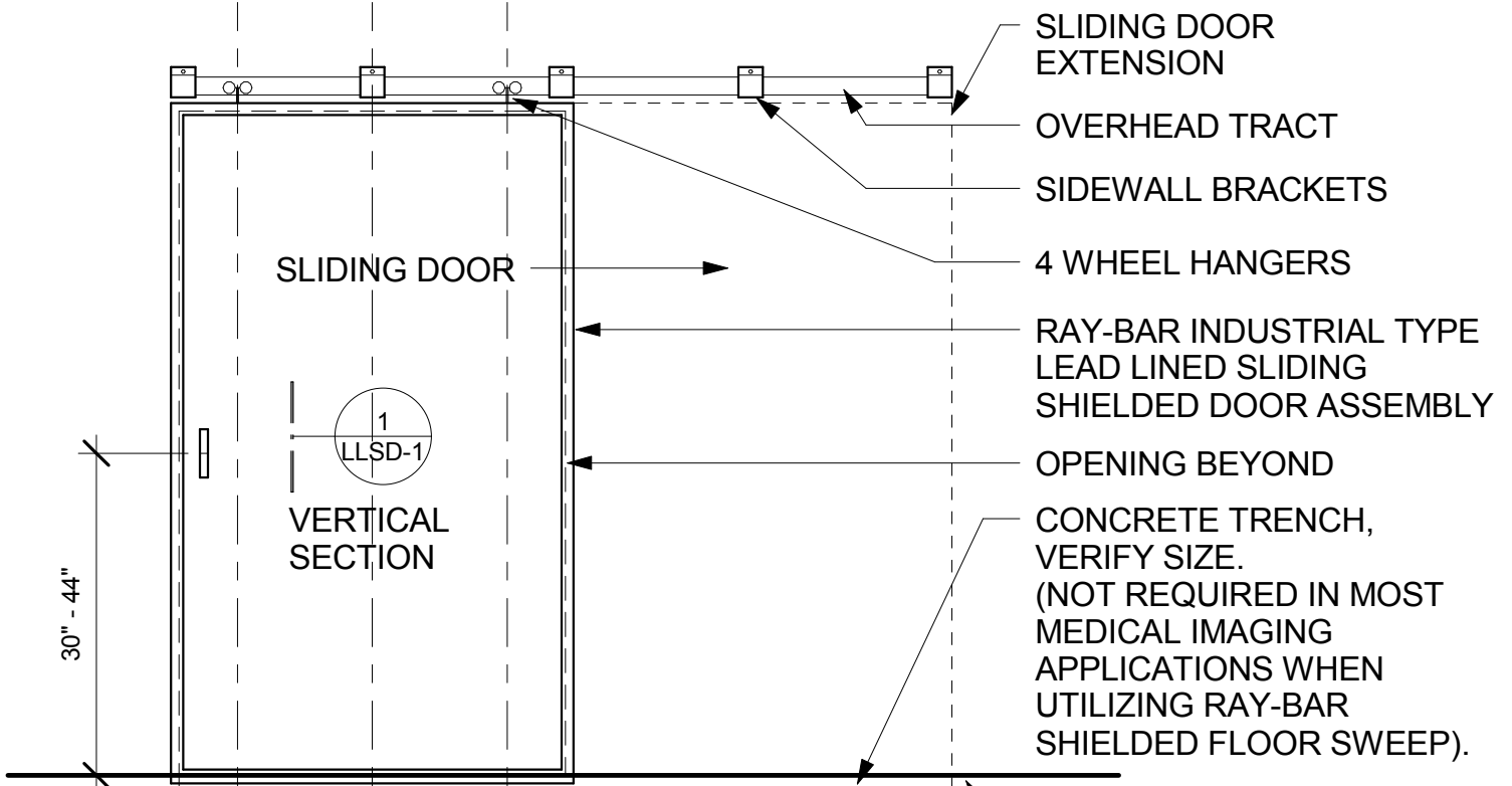
① RAY-BAR INDUSTRIAL LEAD LINED DOOR - SINGLE 1/2" = 1'-0"
